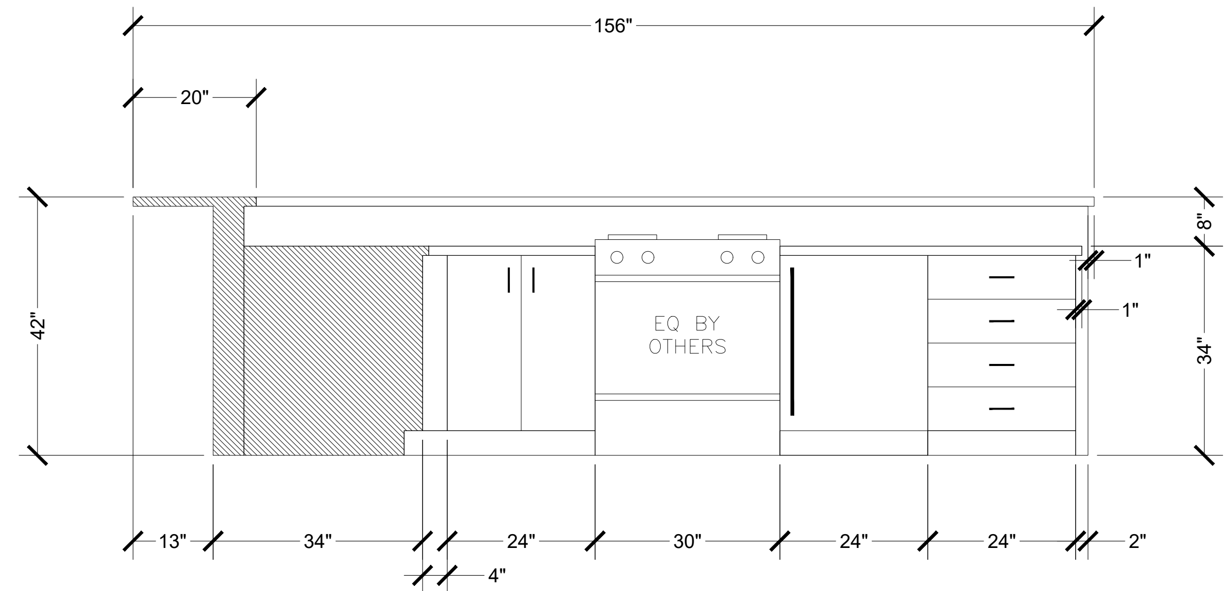
2 ELEVATION - KITCHEN Scale: 3/4" = 1'-0" X/X
