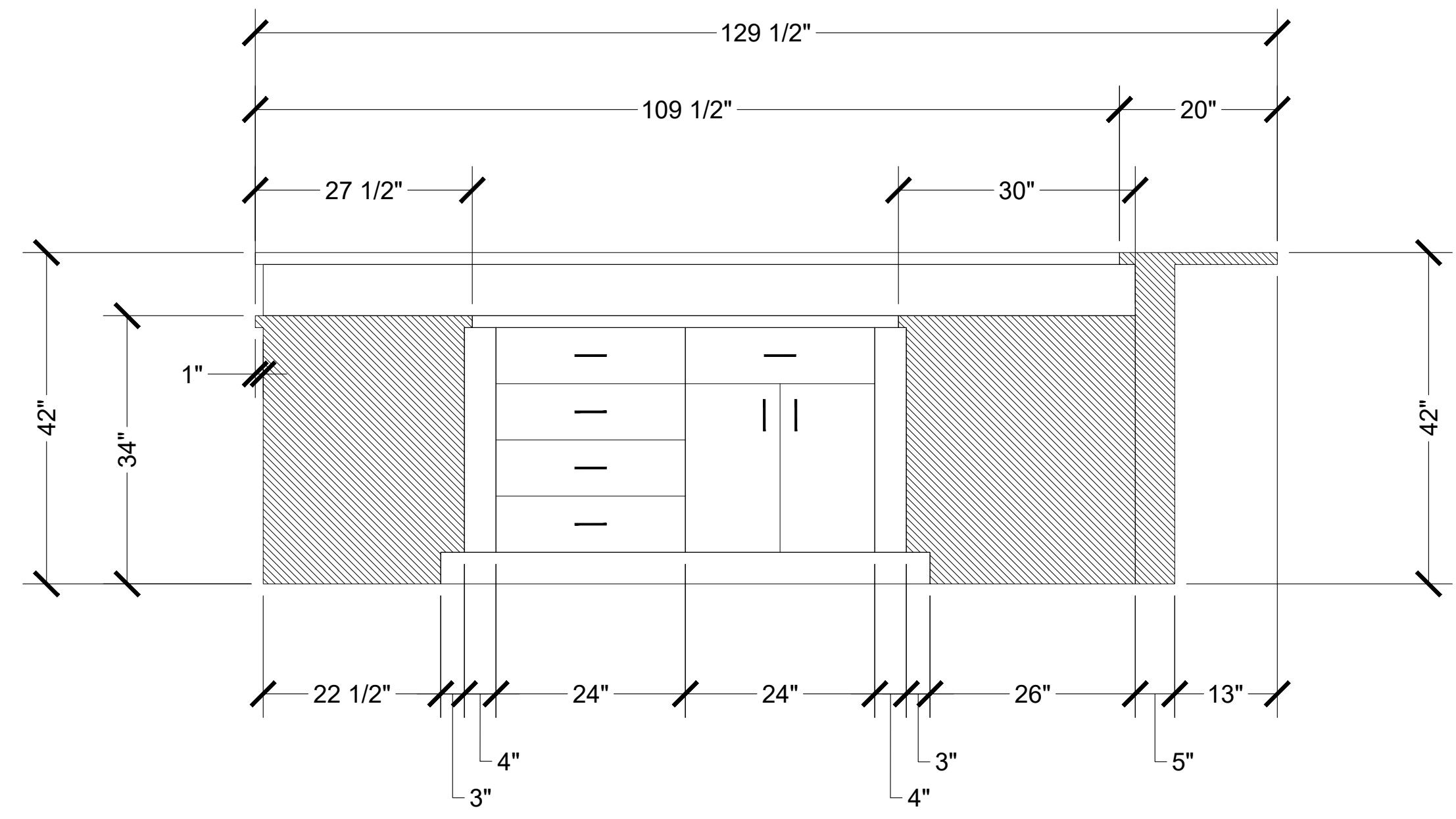
1 ELEVATION - KITCHEN Scale: 3/4" = 1'-0" X/X
